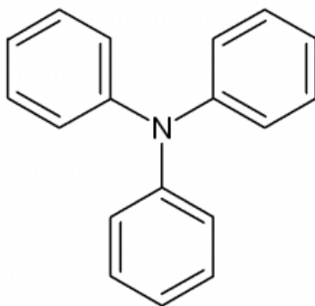
Triphenylamine
